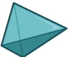
Triangular Pyramid
