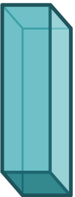
Rectangular Prism
