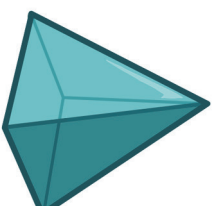
Square Pyramid
