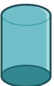
Cylinder
