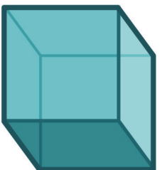
Cube
