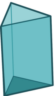
Triangular Prism
